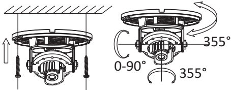
Figure 2-2 3-axis Adjustment
